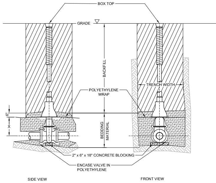
# STANDARD GATE VALVE BOX SETTING C### NTS
