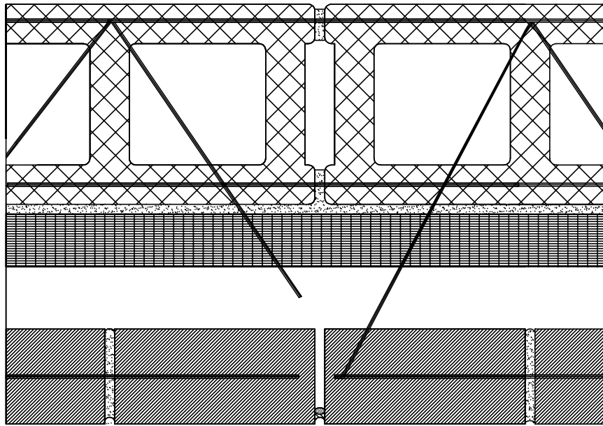
CONTINUOUS TRUSS TYPE REINFORCING
