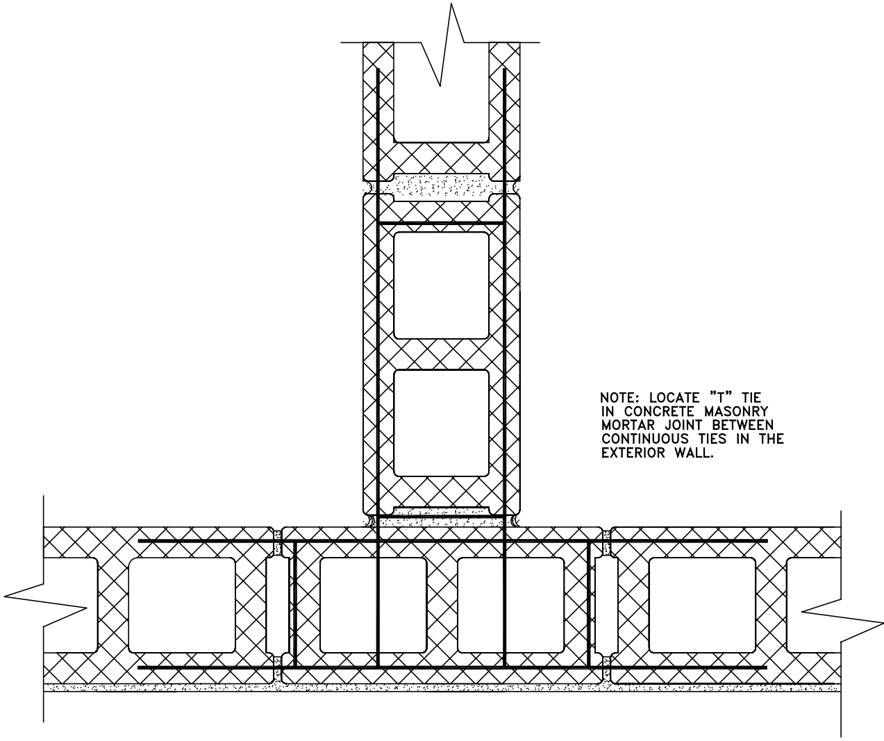
EXTERIOR WALL / CROSS WALL JUNCTURE DETAIL
