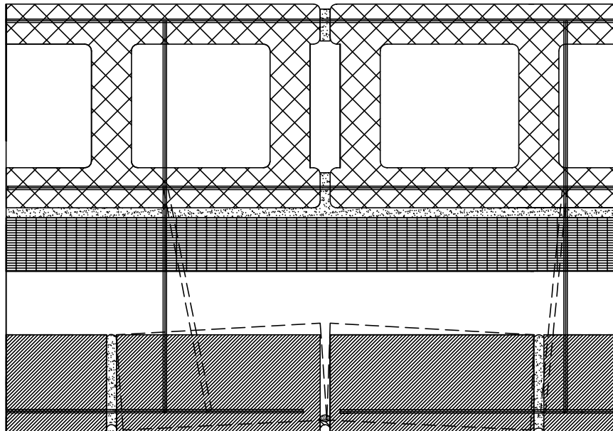
CONTINUOUS LADDER TYPE REINFORCING
