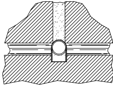
ELEVATION AT WEEP - VENT
