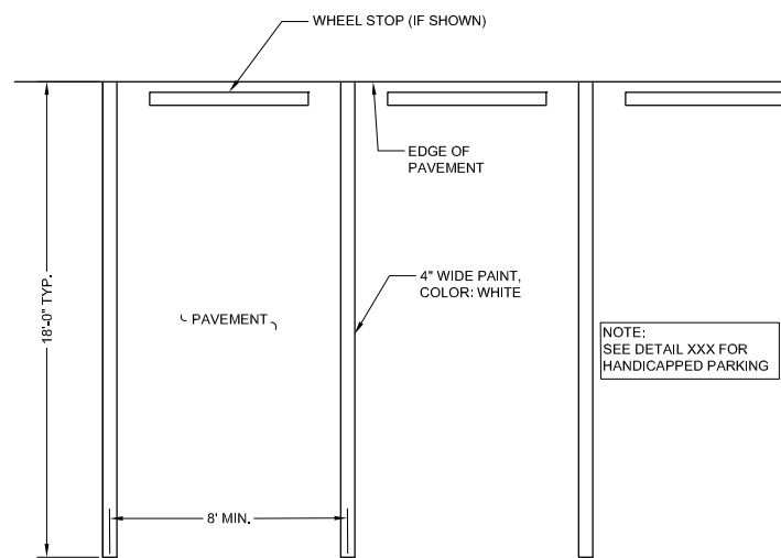
# PARKING STRIPING C### NTS
