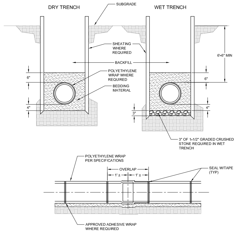
# STANDARD WATER MAIN TRENCH SECTION NTS C###
