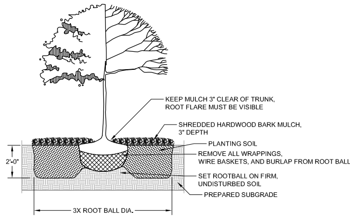
# DECIDUOUS TREE PLANTING WITH MULCH RING C### NTS
