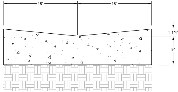
# CONCRETE FLUME C### NTS
