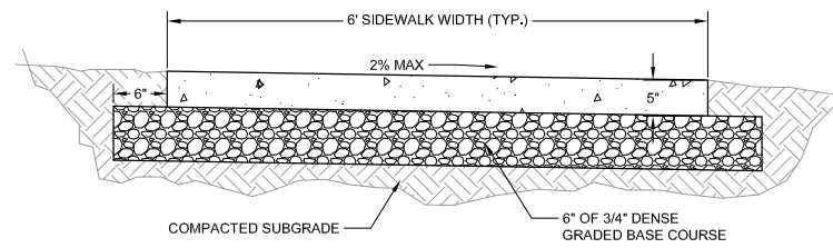
TYPICAL SECTION
