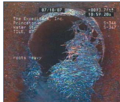
Sanitary Sewers
